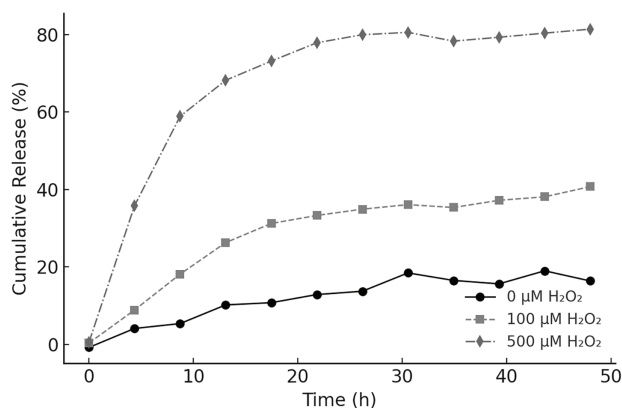
Figure 5. Cumulative NGF release from PCL–PTK–PCL nanocarriers under different oxidative conditions. The release profiles were measured in PBS containing 0, 100 μM, and 500 μM H 2 O 2 at 37°C. The release rate was strongly dependent on the ROS concentration, with rapid NGF liberation observed at elevated H 2 O 2 levels, confirming the oxidation-triggered degradability of the thioketal linkage within the polymer matrix
